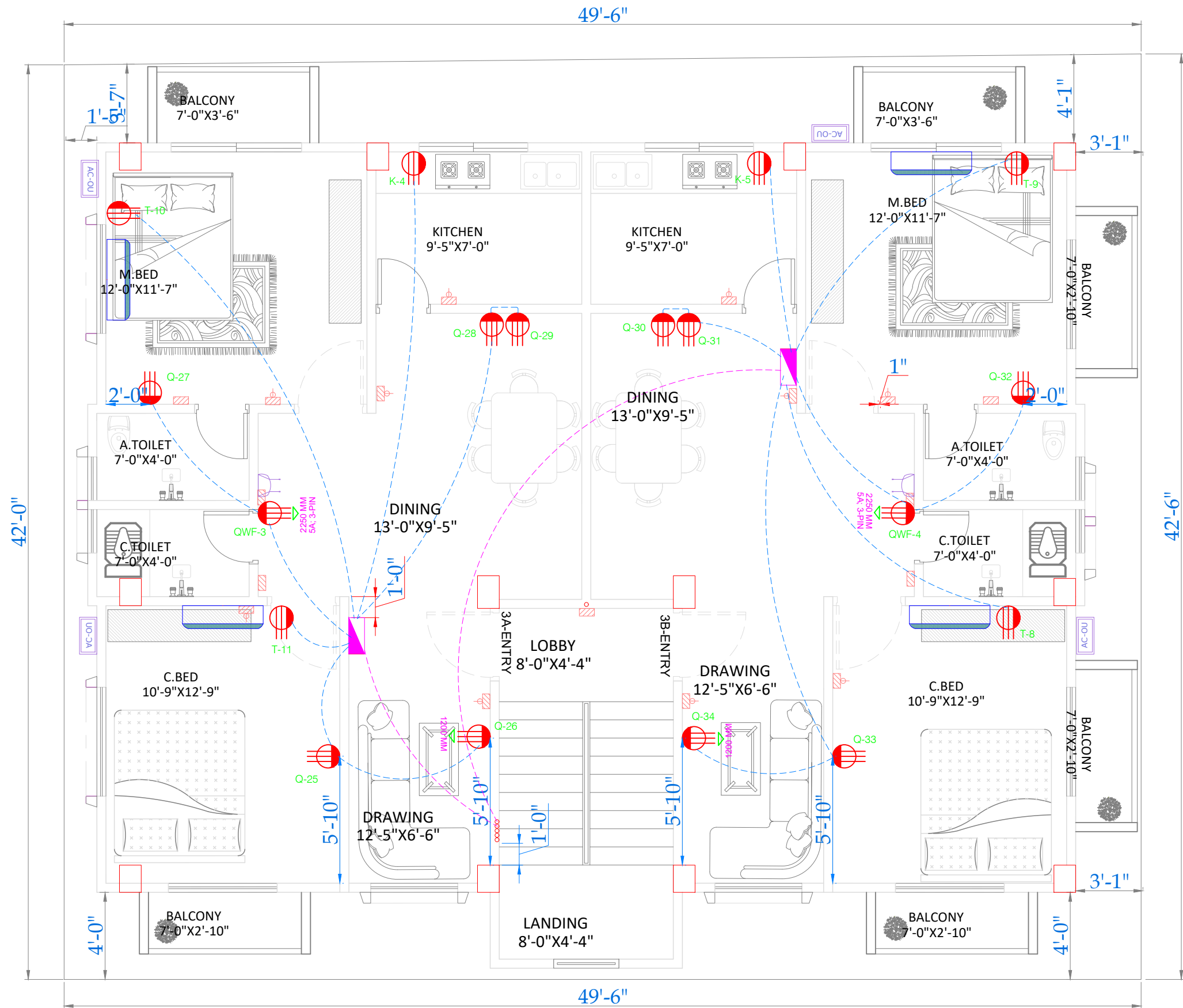
2ND & 3RD FLOOR POWER CIRCUIT PLAN SCALE 5":1'
