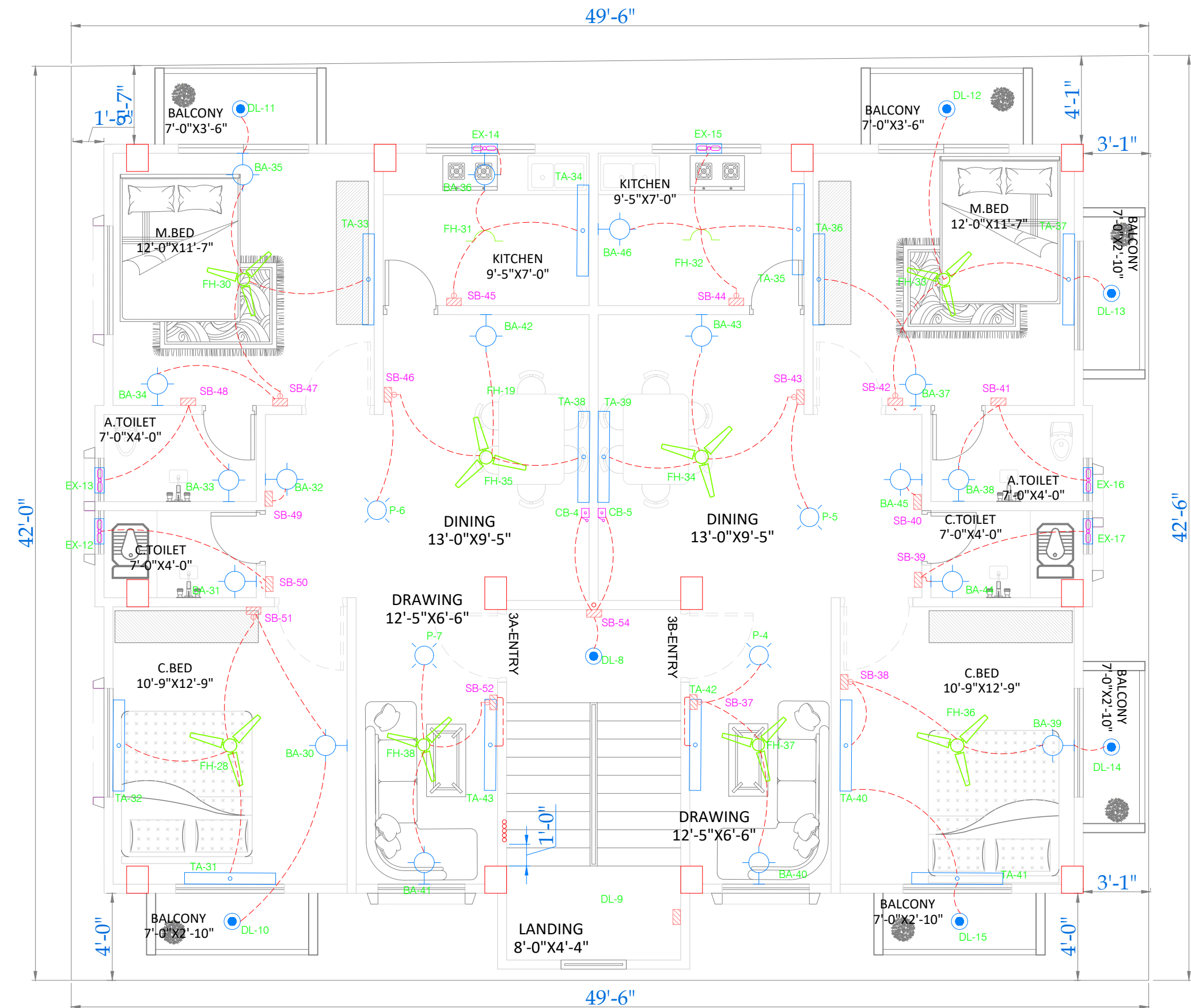
2ND & 3RD FLOOR LIGHTING FIXTURE COUNDUET PLAN SCALE 5":1'
