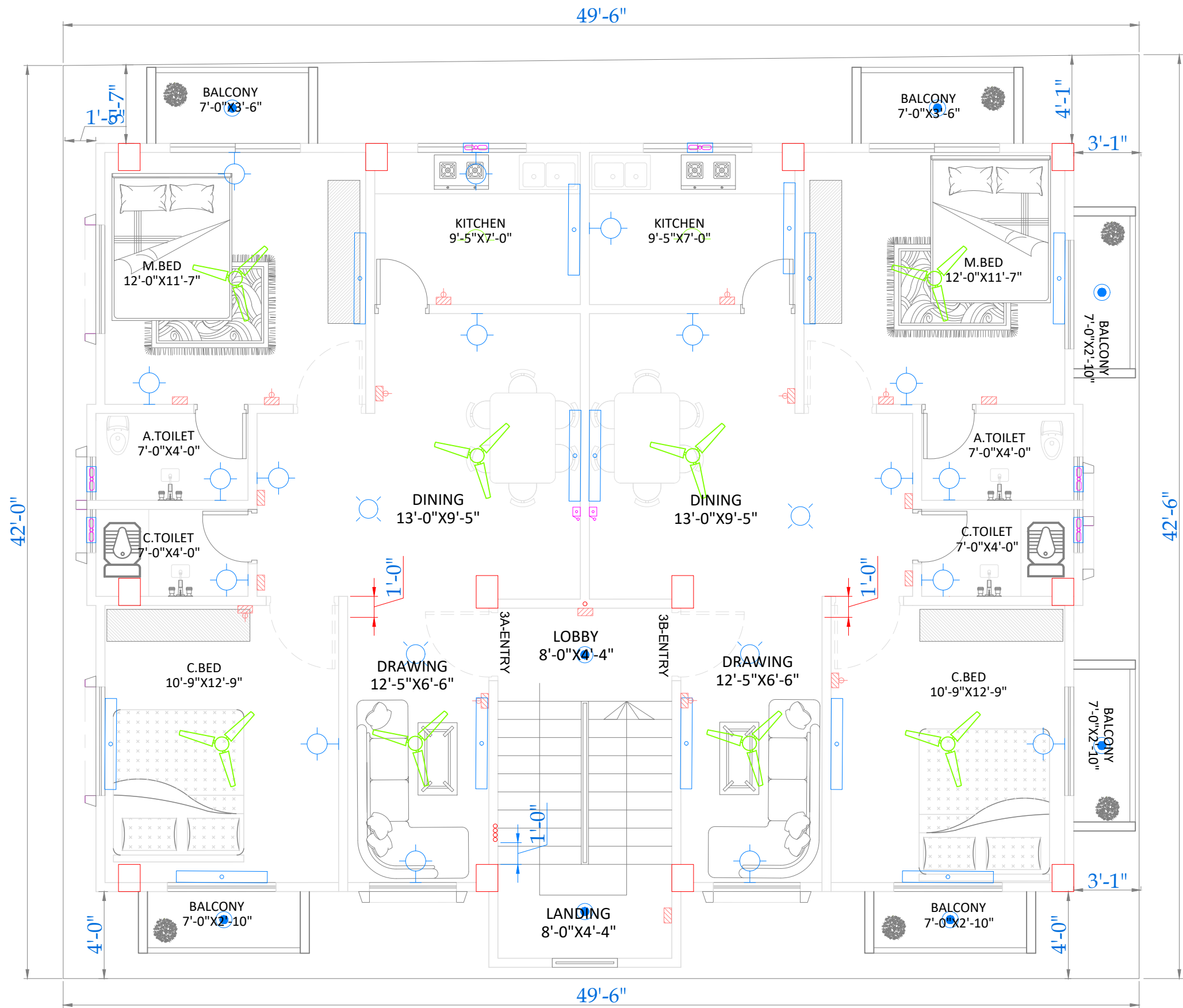
2ND& 3RD FLOOR FIXTURE PLAN SCALE 5":1'
