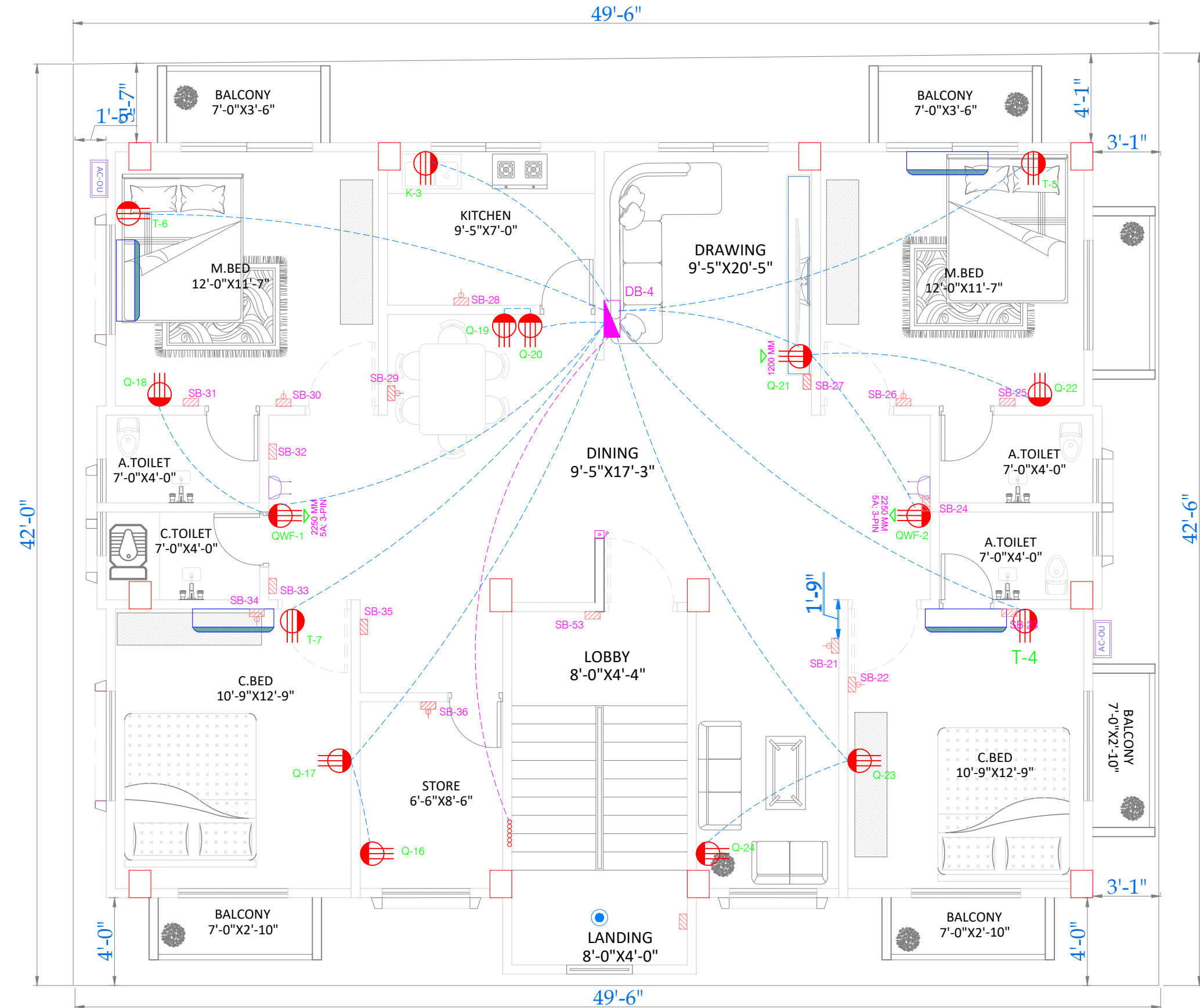
1ST FLOOR (1 UNIT) POWER CIRCUIT PLAN SCALE 5":1'
