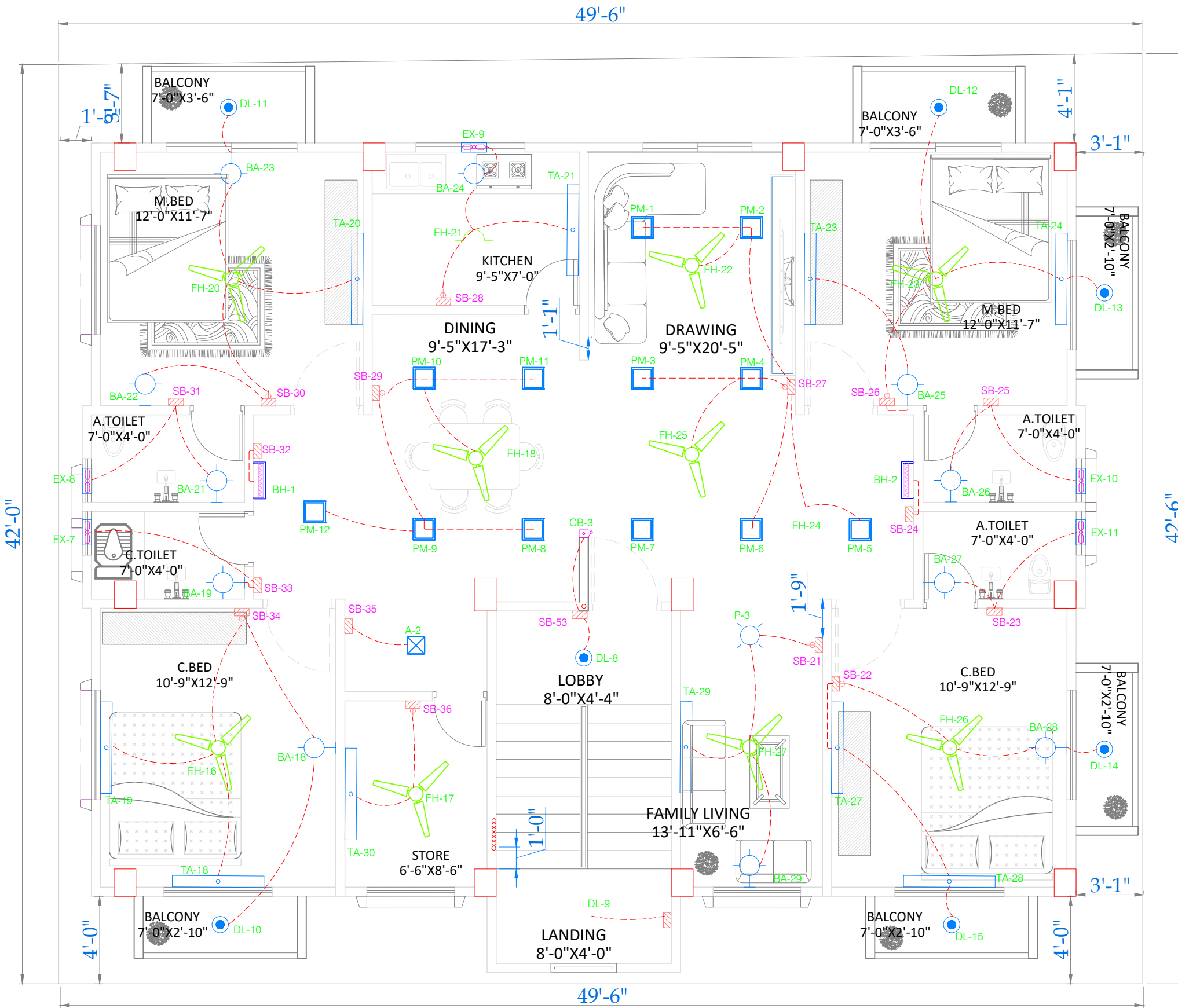
1ST FLOOR (1 UNIT) LIGHTING FIXTURE COUNDUET PLAN SCALE 5":1'
