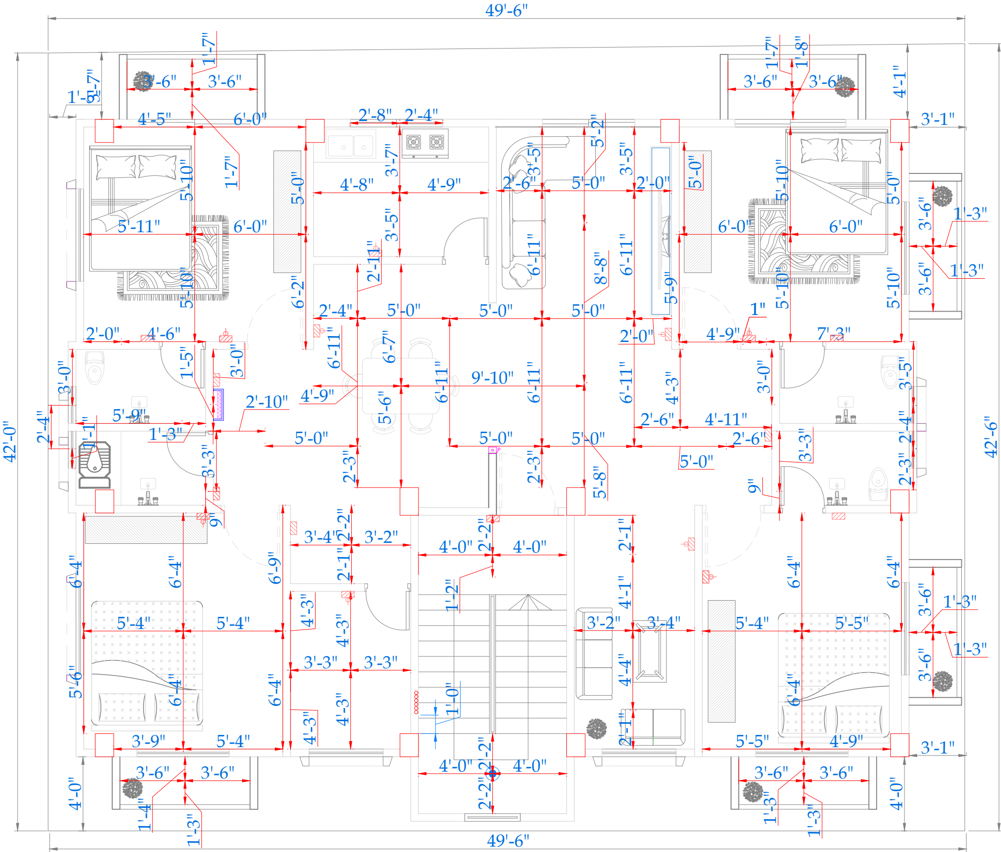
1ST FLOOR (1 UNIT) FIXTURE DIMENSION PLAN SCALE 5":1'
