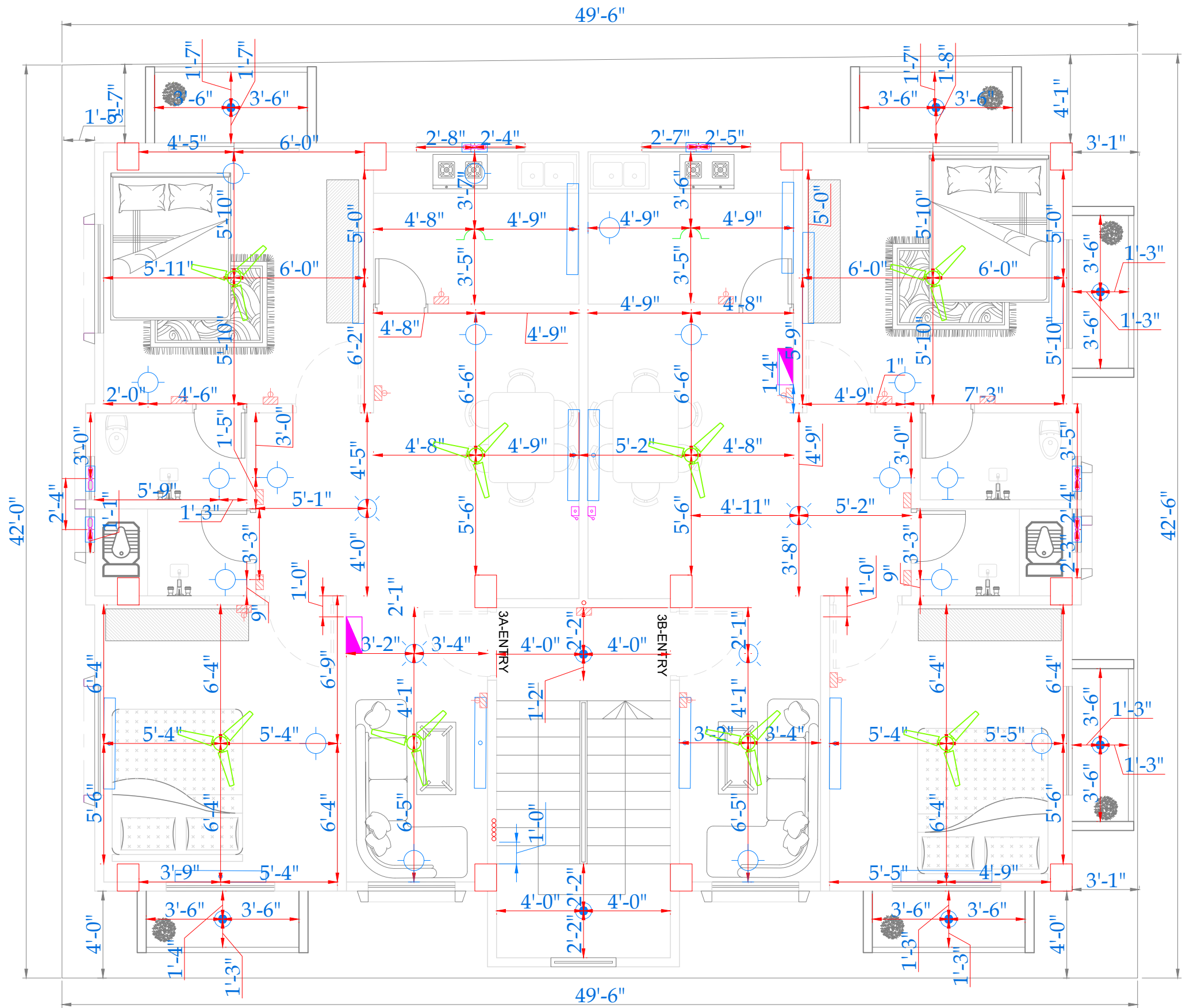
2ND & 3RD FLOOR FIXTURE DIMENSION PLAN SCALE 5":1'
